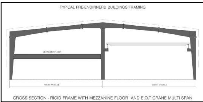
MEZZANINE FLOOR & E.O.T CRANE MULTI SPAN
